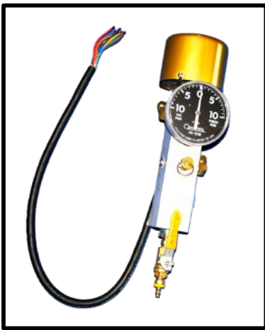
Gauge Switch Manifold
