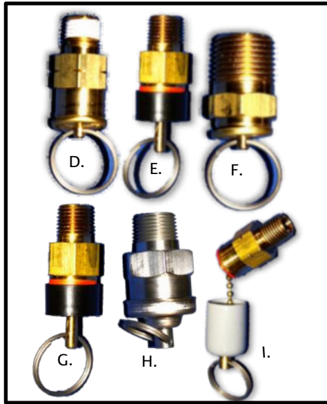
Part # 205-001-01 10 PSI 1 1/4" Thread
